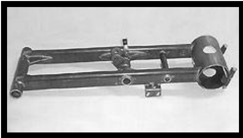
Banshee Swingarm Shown in bare metal. Oval tubing / round housing $399.00
