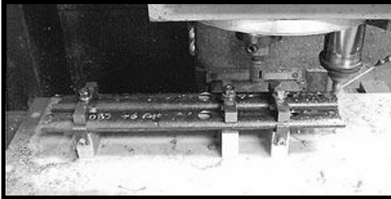
CNC milled tubing and carrier housings Decreased labor costs and increased accuracy
