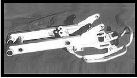
Blaster Swingarm Shown with opt. powder coating. Square tube / standard housing $429.00 Skid plate mounts incorporated in the design.
